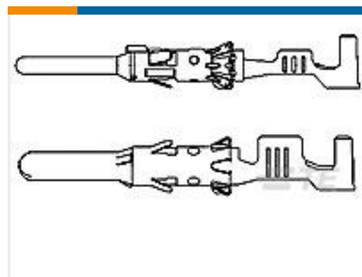
TE Part # 962972-8 2,5MM PIN CONTACT LP (>1,0-2,5) SWS
